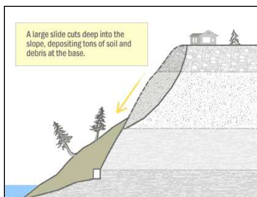
Figure 13-4. Large Slide
